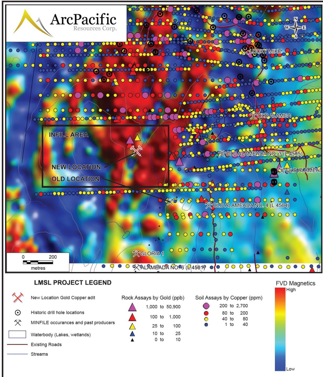
Figure 2: Lucky Mike Area on the LMSL Property, showing the new properly located and old improperly plotted location of historic gold copper mine over first vertical magnetics, copper in soils (ppm) and gold in rocks (ppb).
