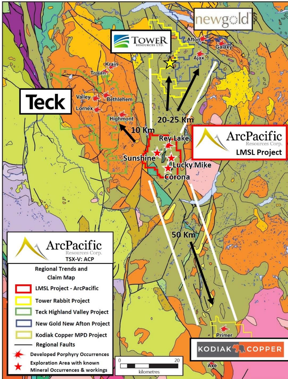
Figure 3: Location Map of ArcPacific’s LMSL Property over regional geology showing mineralized trend and other notable projects.
